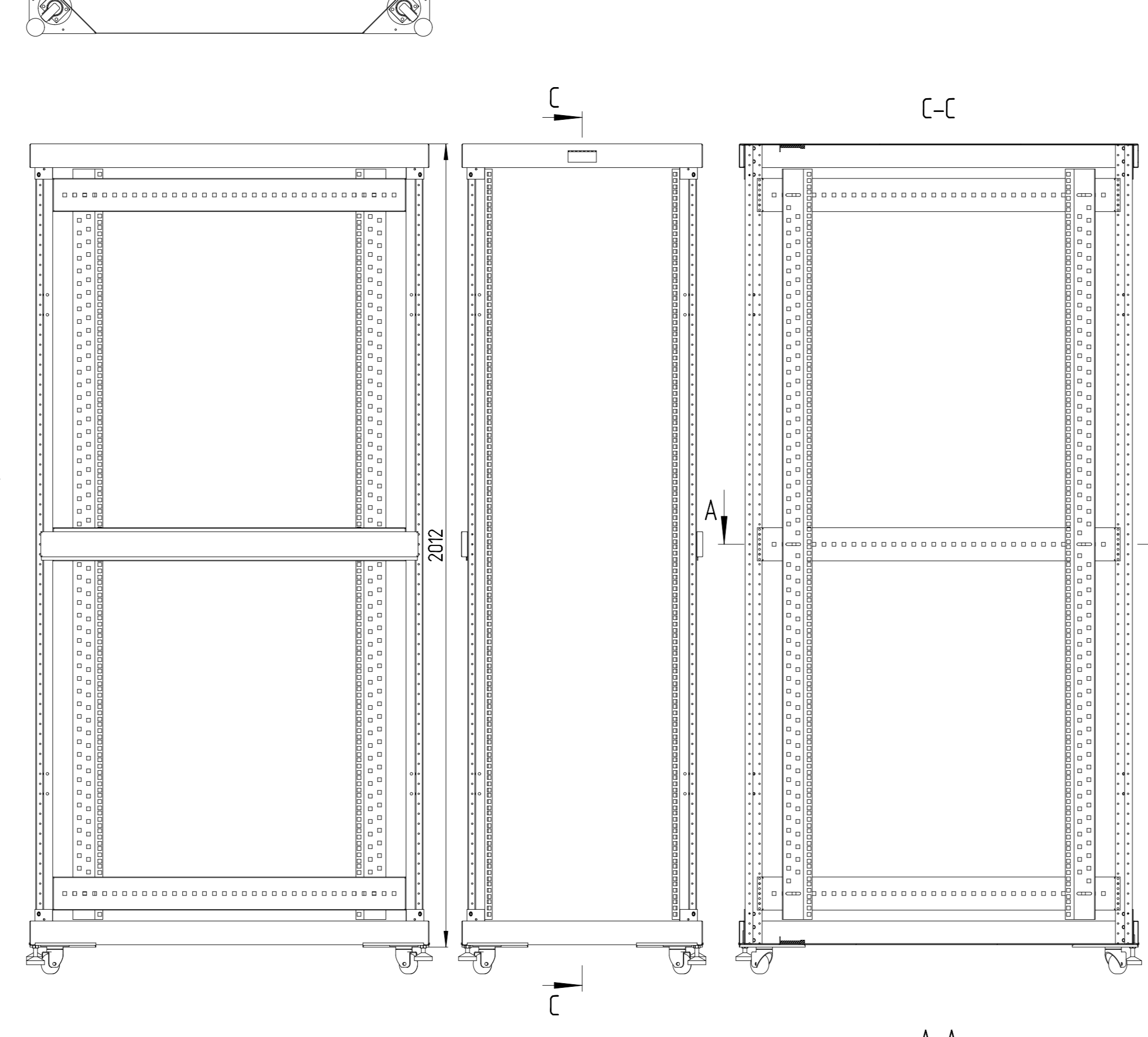
19" cabinet for IT 42U 600x1000x2010 TR 6042*** (Scale 1:10)
