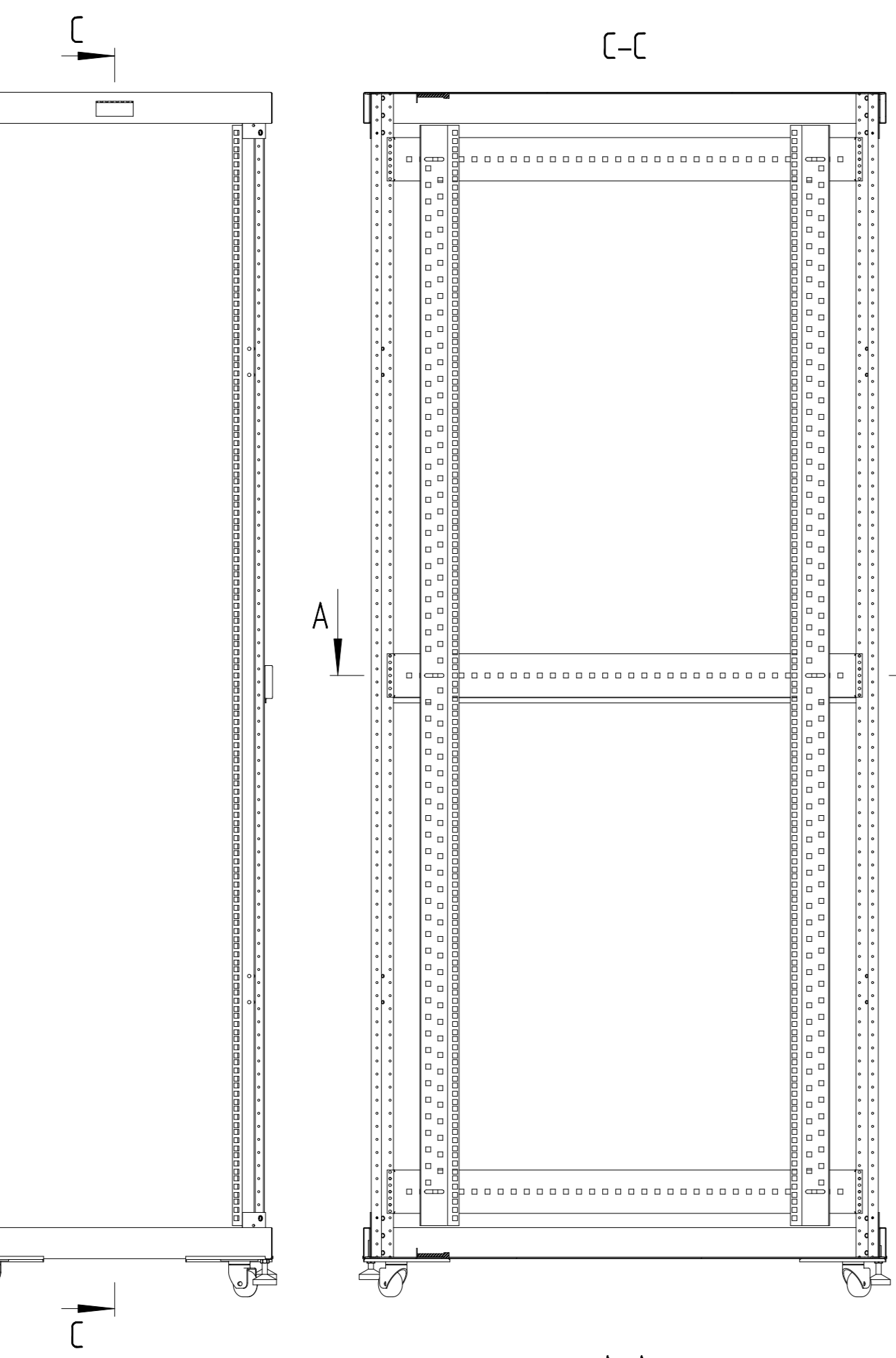
19" cabinet for IT 47U 600x1000x2230 TR 6047*** (Scale 1:10)
